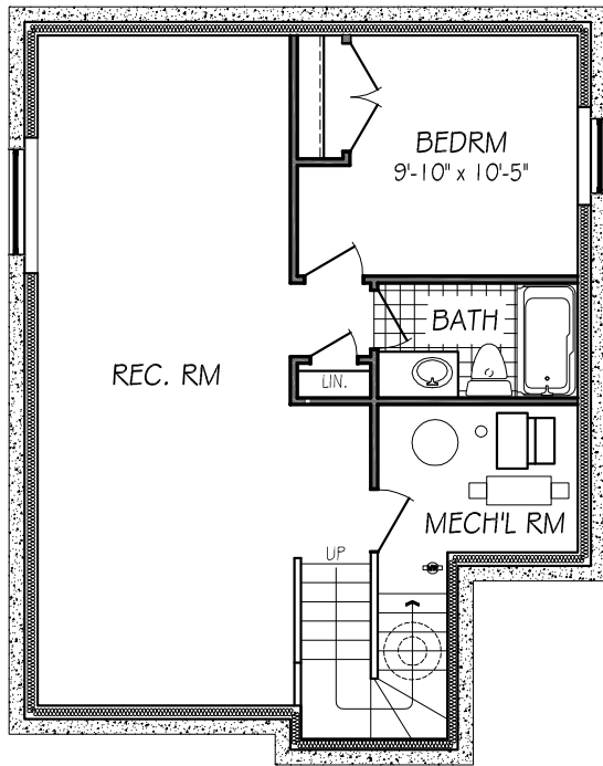
OPT'L LOWER LEVEL DEV. PLAN 546 SQ. FT.
