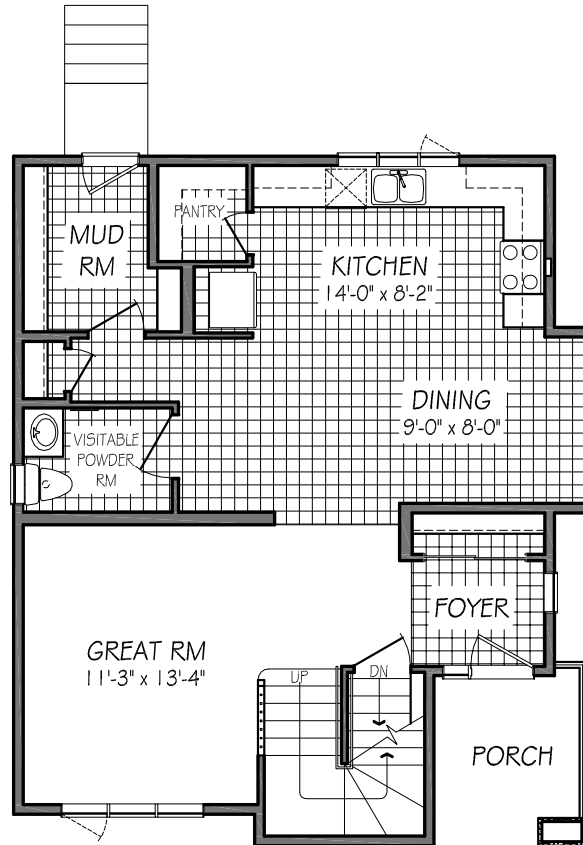
MAIN FLOOR PLAN 815 SQ. FT.
