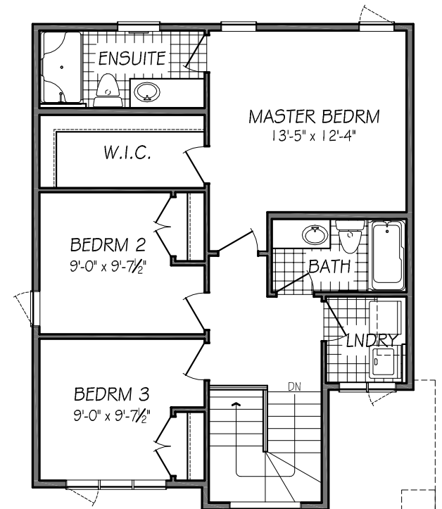
SECOND FLOOR PLAN 797 SQ. FT.
