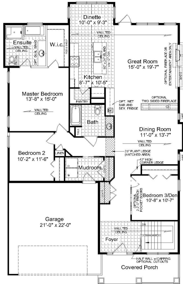
Main Floor Plan 1910 sq. ft.
