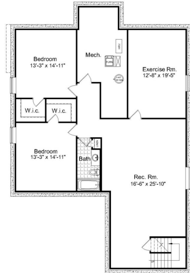
Optional Basement Layout 1447 Sq. ft. (approx. finished space)
